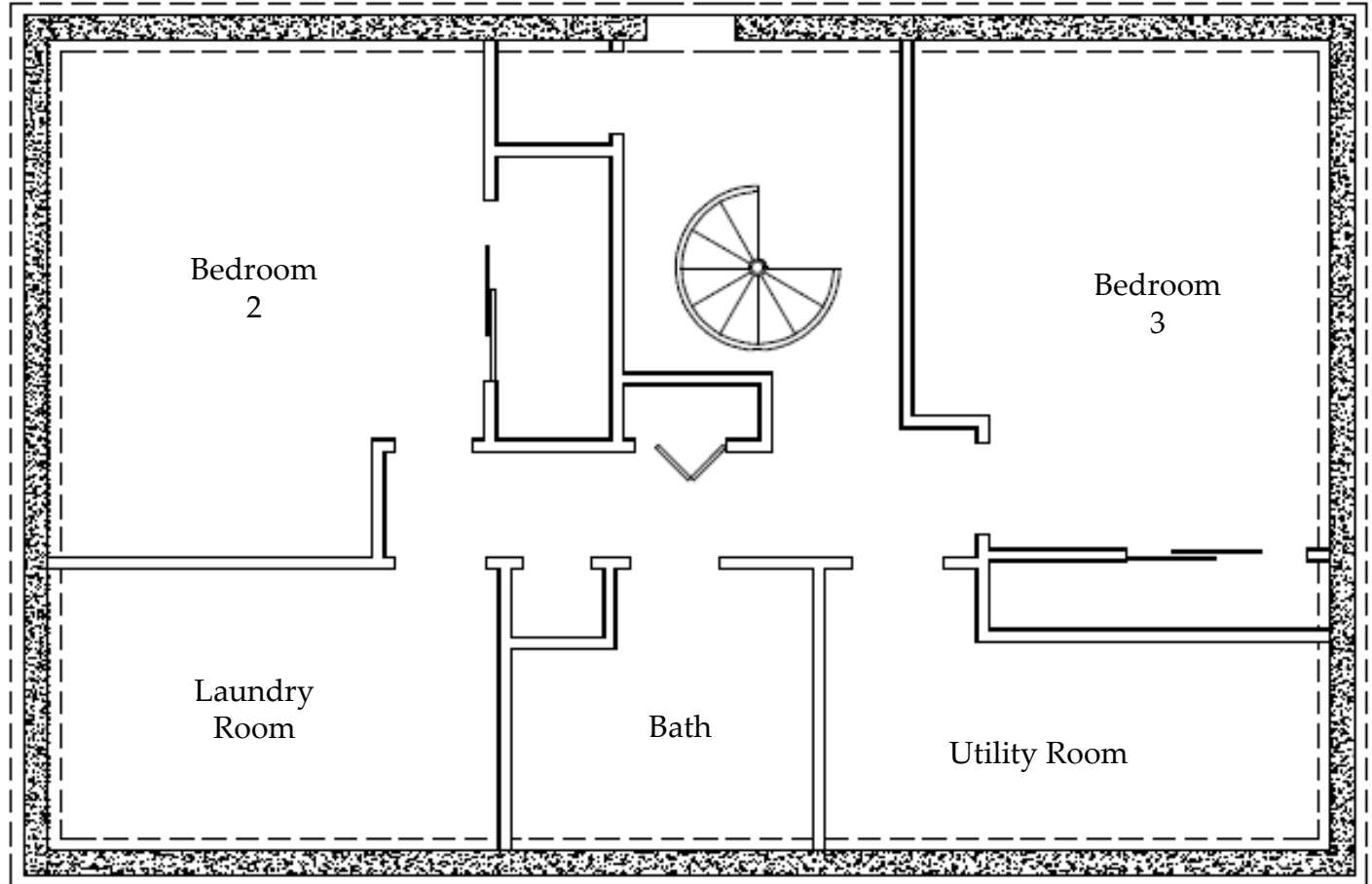
Guest House Lower Level
